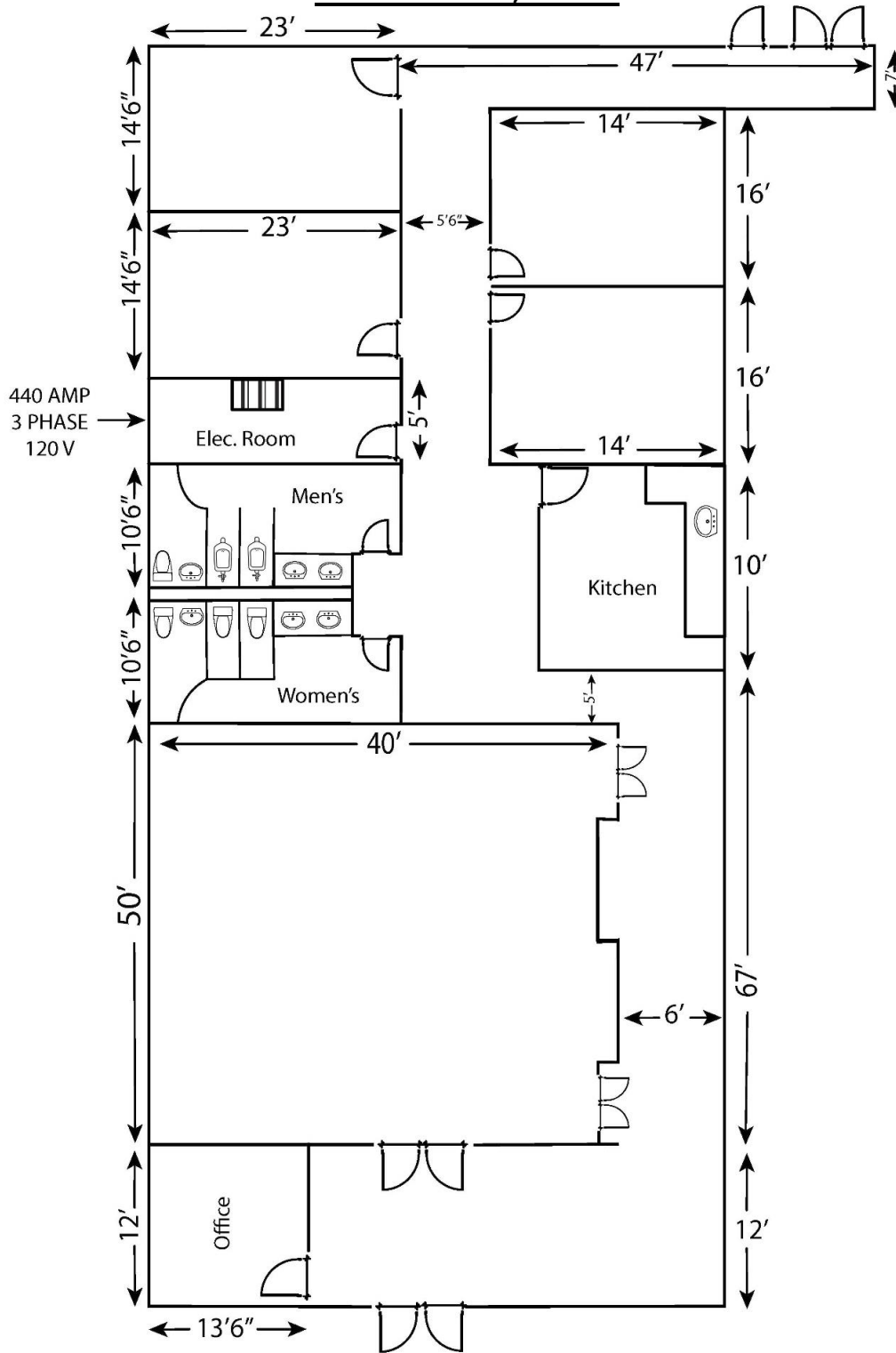
Floor Plan- 5,532 SF
