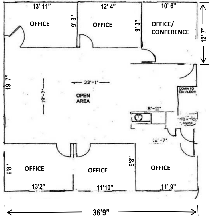
2 nd Floor - 1,500 SF
